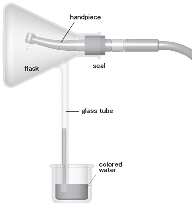
Fig. 1 Complete test setup: Measuring suck-back pressure of the whole handpiece head.
